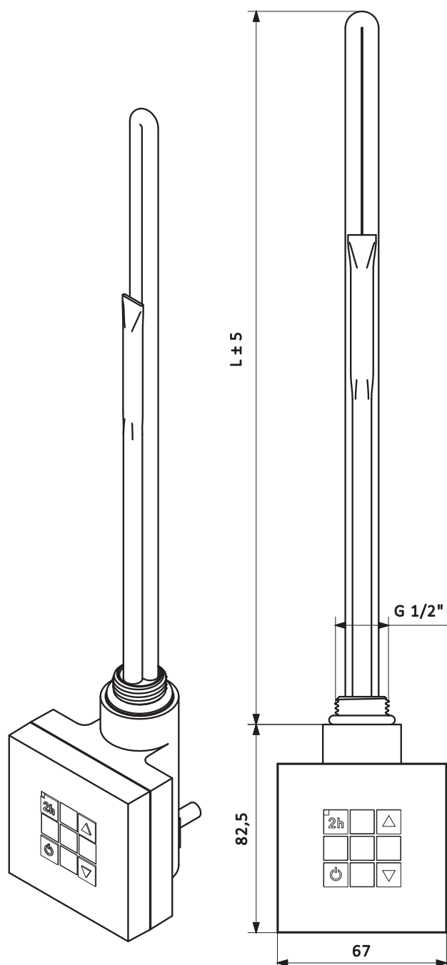
Straight cable with plug. Cable length: 1,5 m
