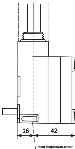
Straight cable with plug. Cable length: 1,5 m
