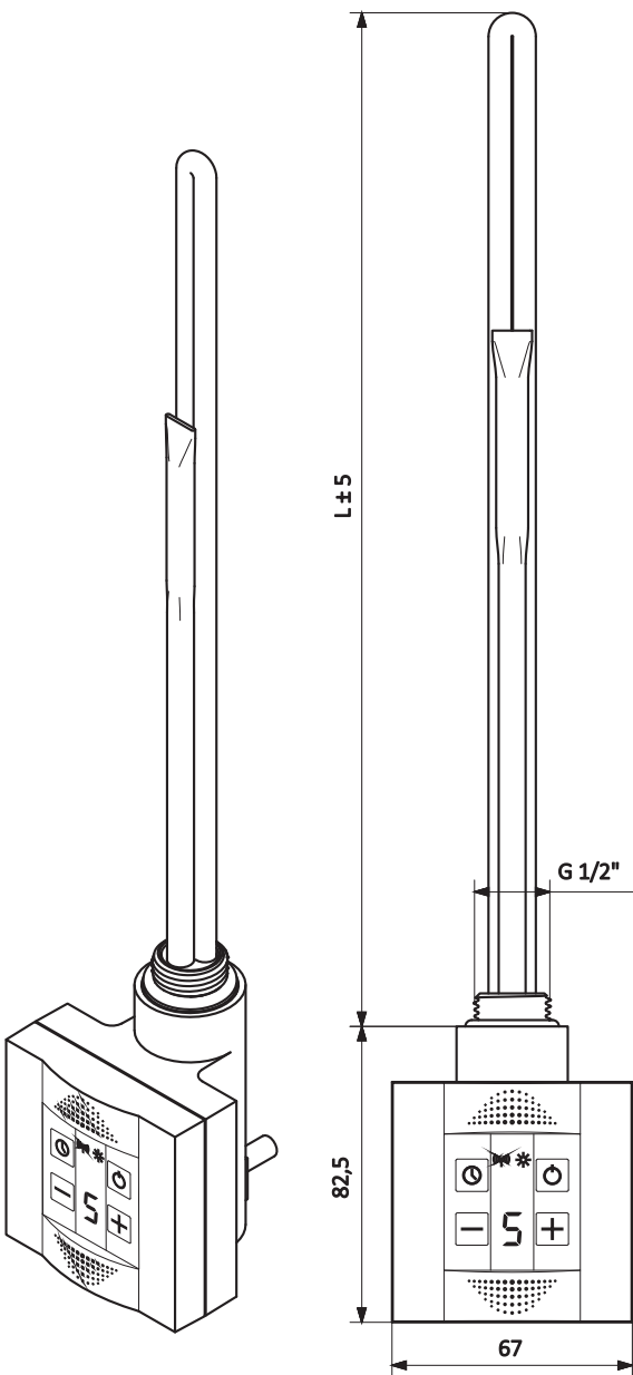
Straight cable with plug. Cable length: 1,5 m
